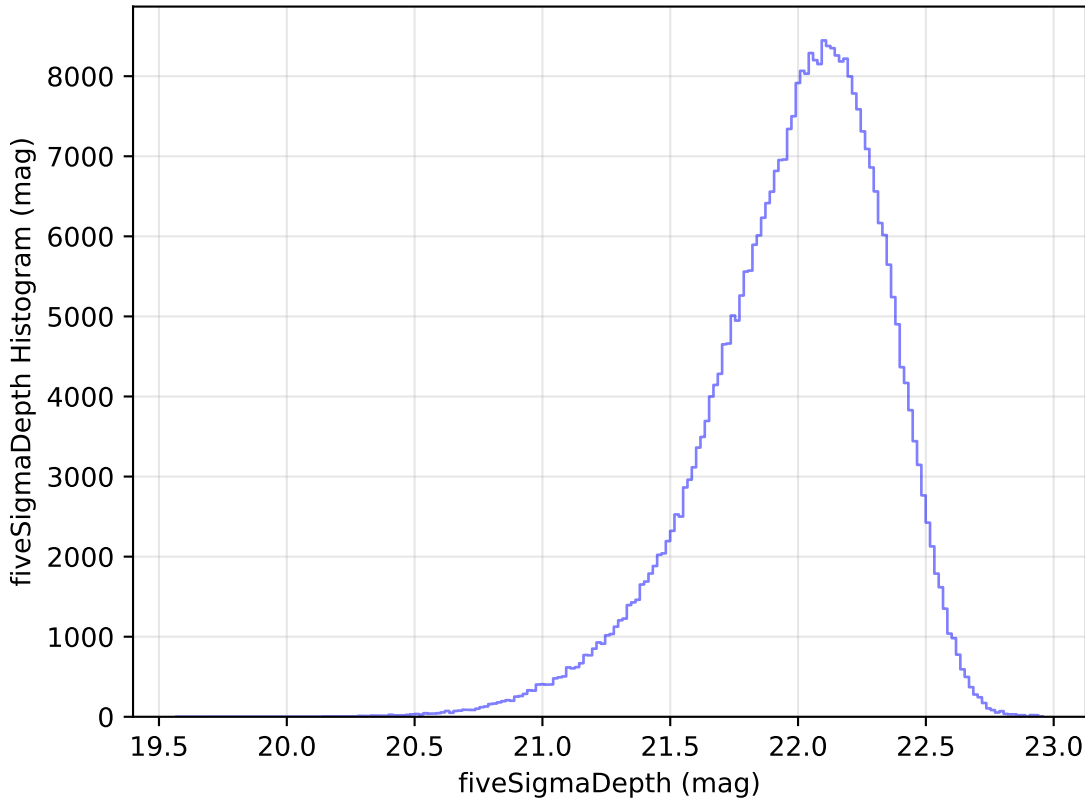
ddf_acor_sf15_ls40_lsr10_v3.4_10yrs All sky y band: fiveSigmaDepth Histogram
