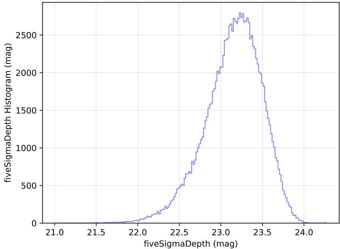
ddf_acor_sf15_lsf40_lsr10_v3.4_10yrs All sky u band: fiveSigmaDepth Histogram
