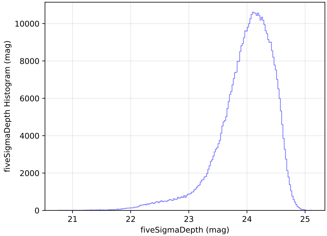
ddf_acor_sf15_lsf40_lsr10_v3.4_10yrs All sky r band: fiveSigmaDepth Histogram
