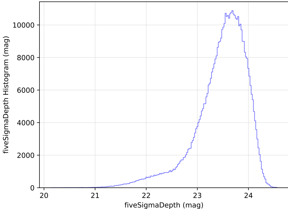
ddf_acor_sf15_lsf40_lsr10_v3.4_10yrs All sky i band: fiveSigmaDepth Histogram
