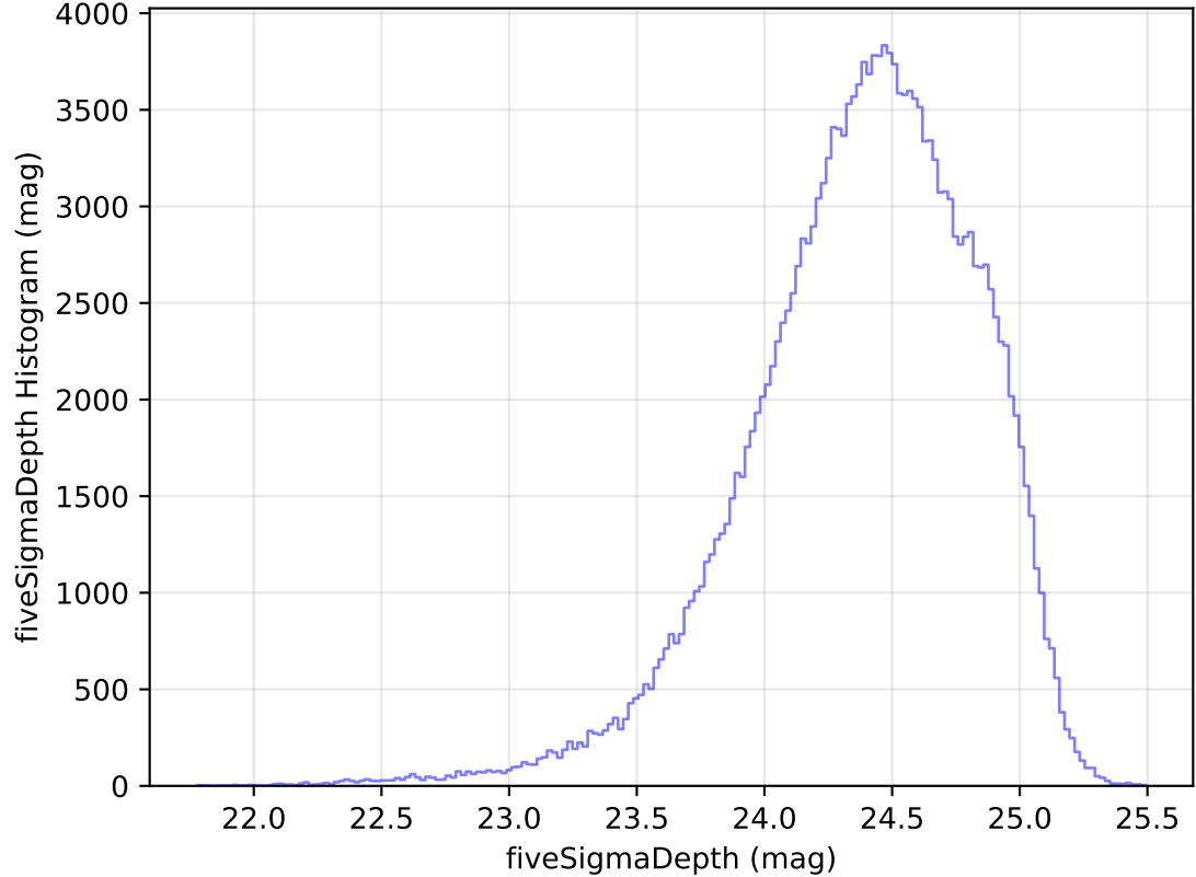
ddf_acor_sf15_lsf40_lsr10_v3.4_10yrs All sky g band: fiveSigmaDepth Histogram
