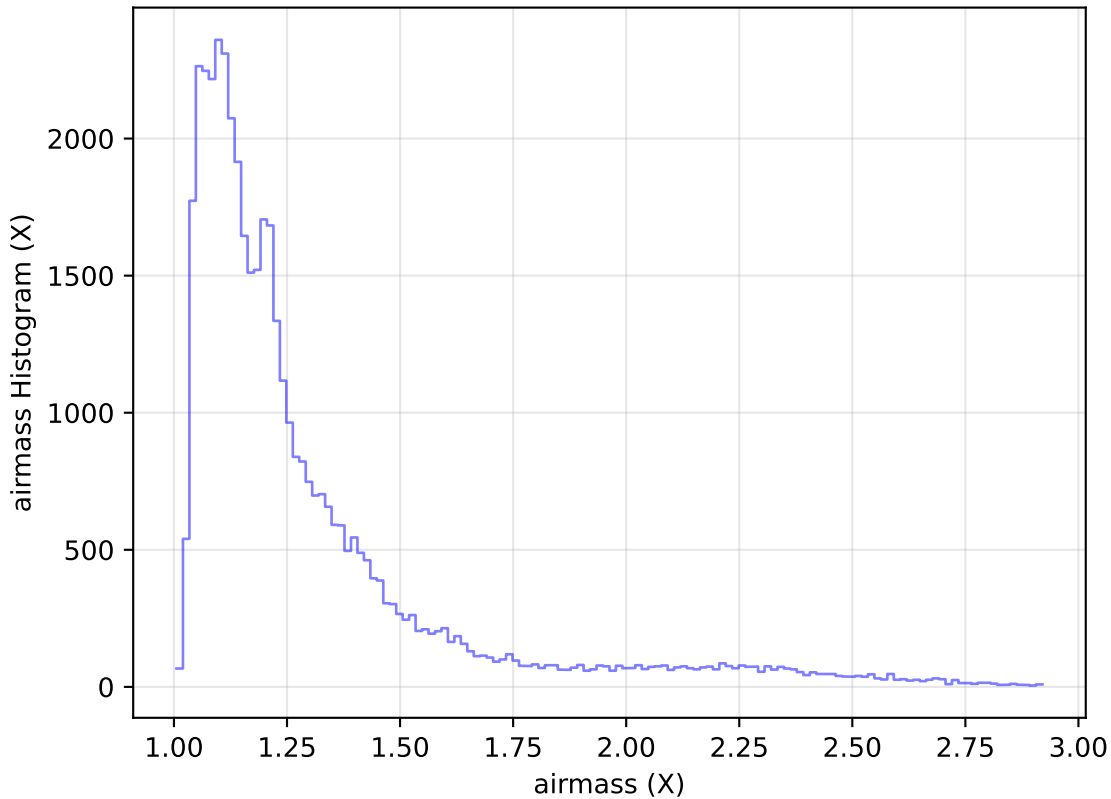
ddf_acor_sf15_lsf40_lsr10_v3.4_10yrs Yr 1 z band: airmass Histogram
