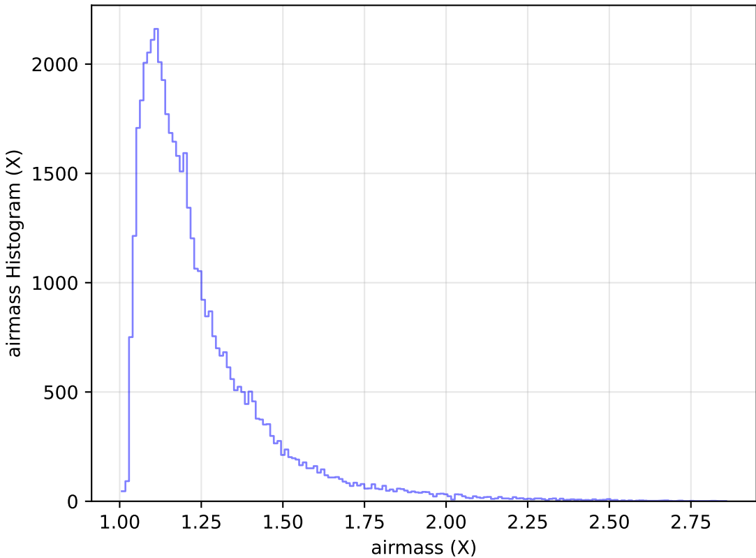
ddf_acor_sf15_lsf40_lsr10_v3.4_10yrs Yr 1 y band: airmass Histogram
