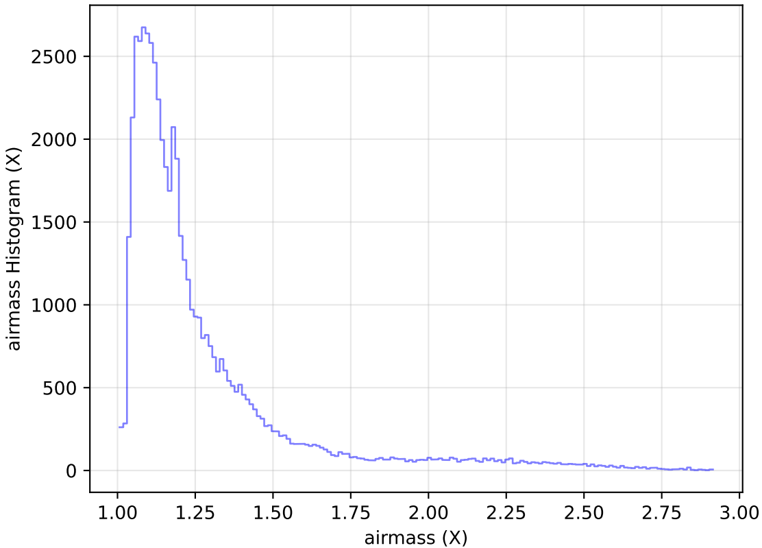
ddf_acor_sf15_lsf40_lsr10_v3.4_10yrs Yr 1 i band: airmass Histogram
