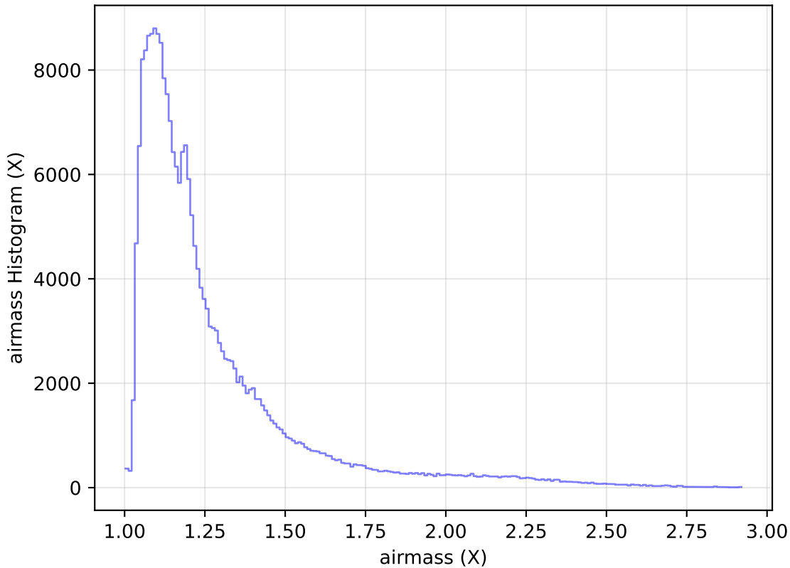
ddf_acor_sf15_lsf40_lsr10_v3.4_10yrs Yr 1 all bands: airmass Histogram
