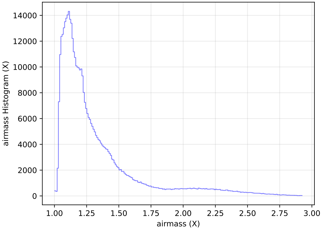
ddf_acor_sf15_lsf40_lsr10_v3.4_10yrs WFD z band: airmass Histogram
