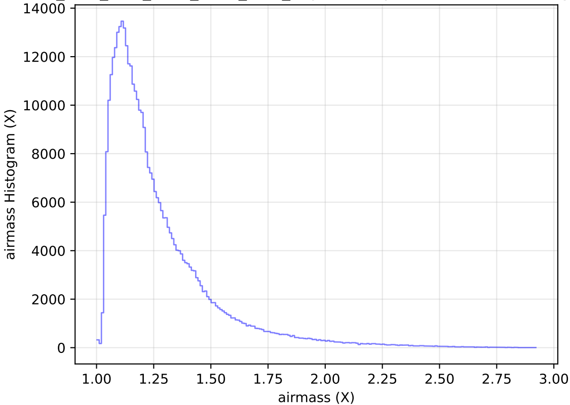
ddf_acor_sf15_lsf40_lsr10_v3.4_10yrs WFD y band: airmass Histogram
