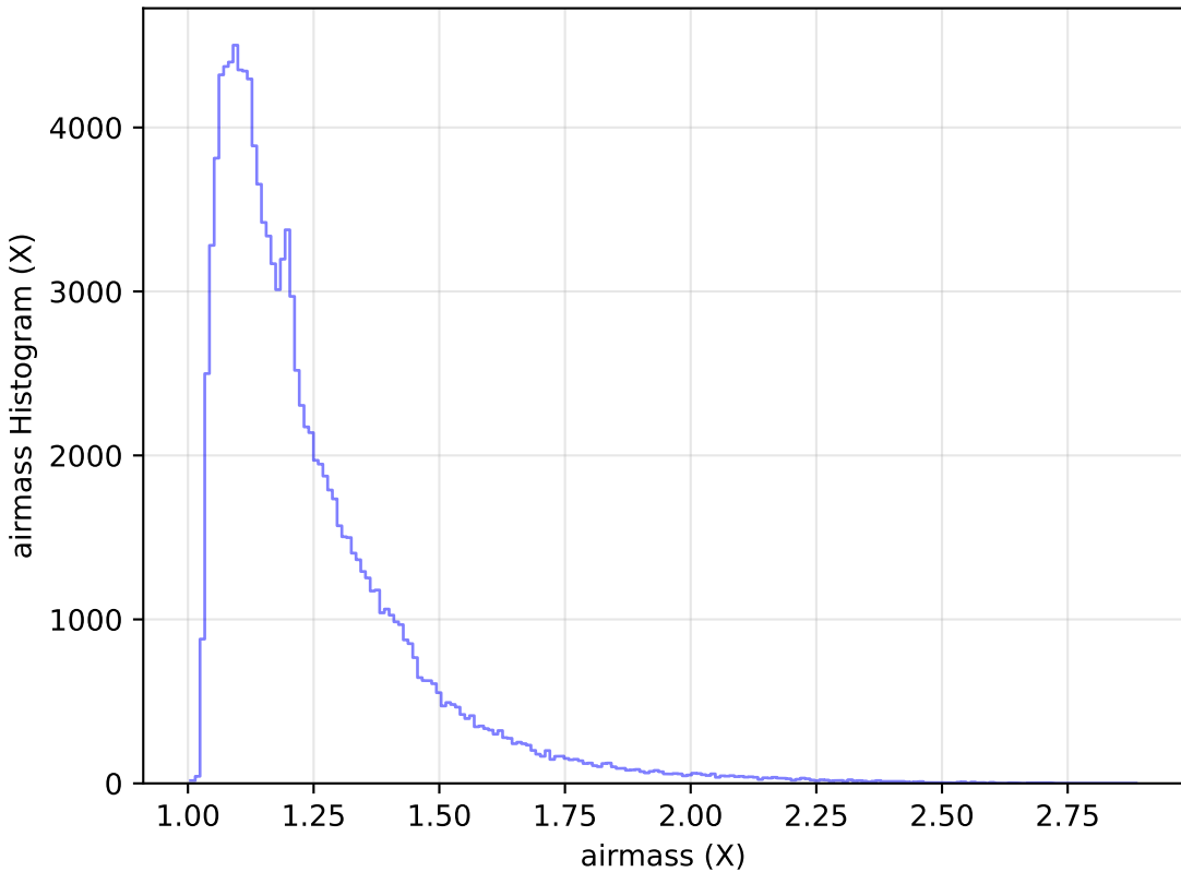
ddf_acor_sf15_lsf40_lsr10_v3.4_10yrs WFD u band: airmass Histogram
