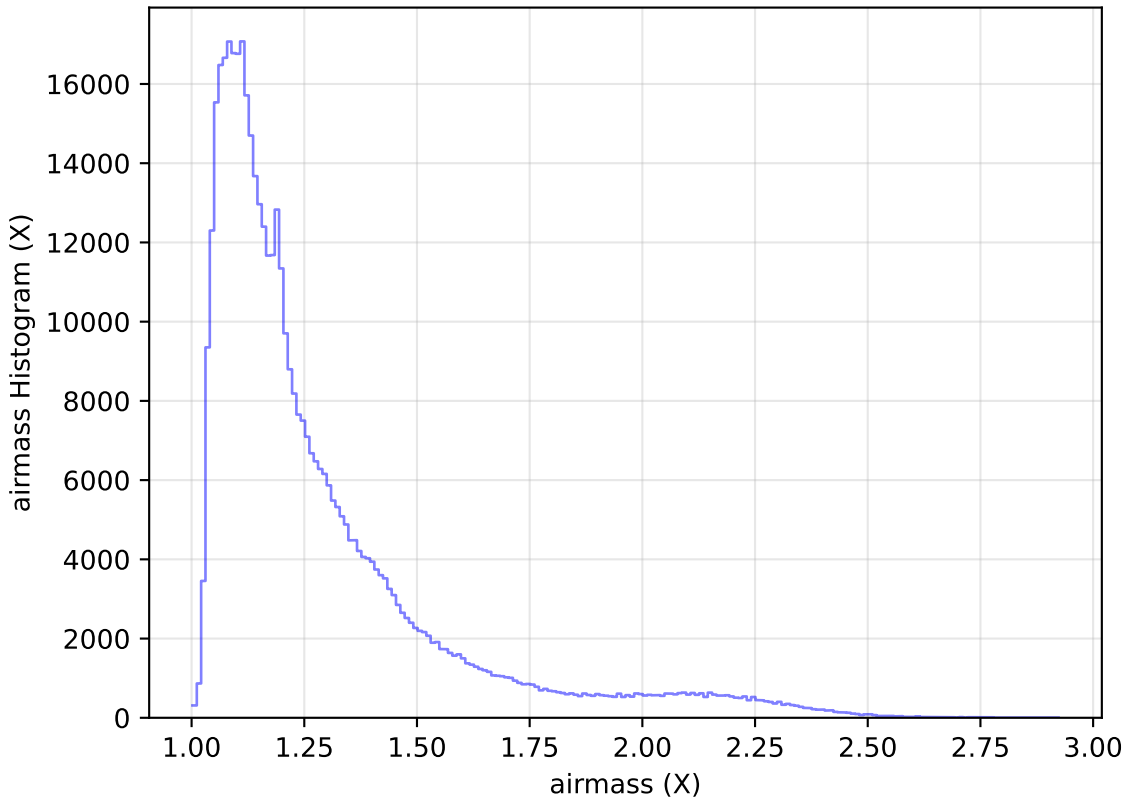
ddf_acor_sf15_Isf40_Isr10_v3.4_10yrs WFD r band: airmass Histogram
