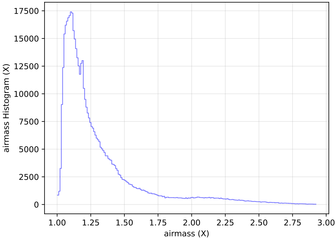
ddf_acor_sf15_lsf40_lsr10_v3.4_10yrs WFD i band: airmass Histogram
