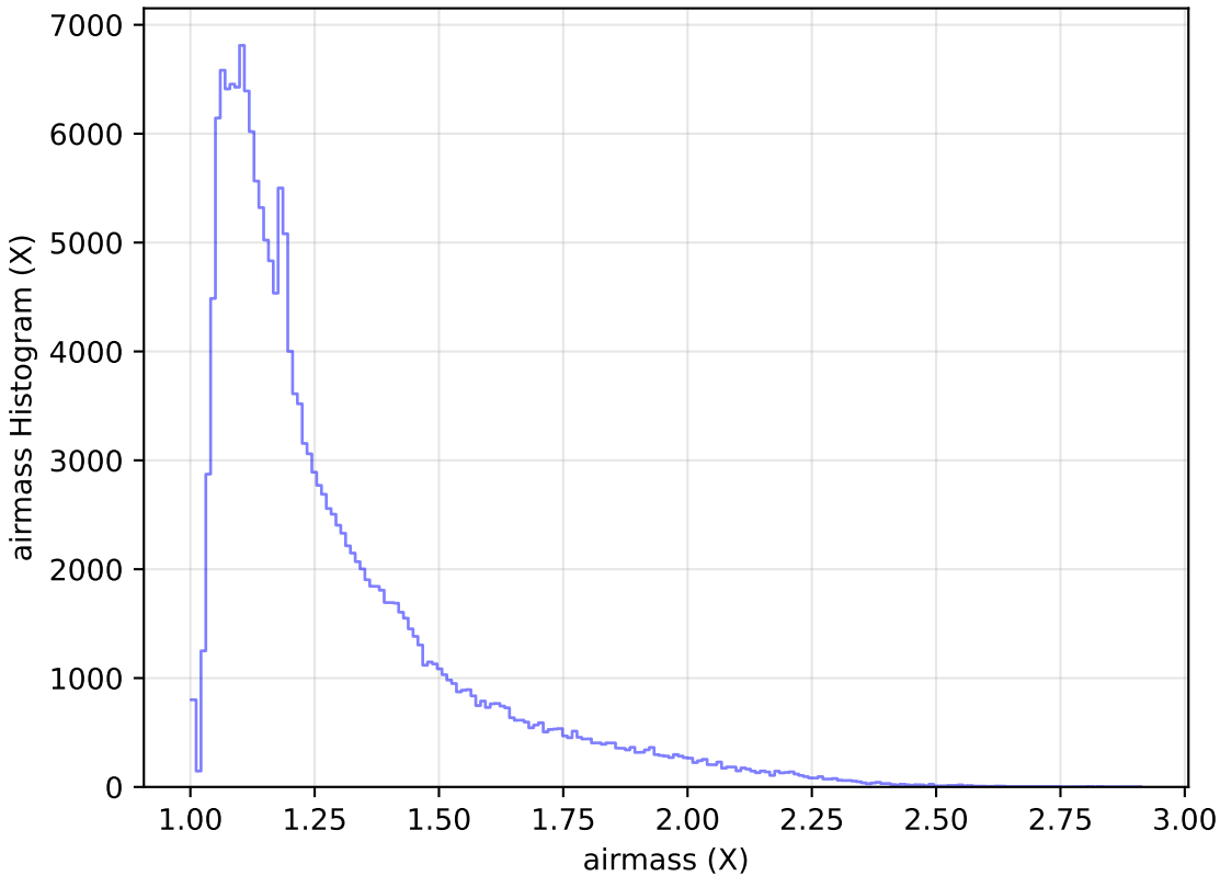
ddf_acor_sf15_lsf40_lsr10_v3.4_10yrs WFD g band: airmass Histogram
