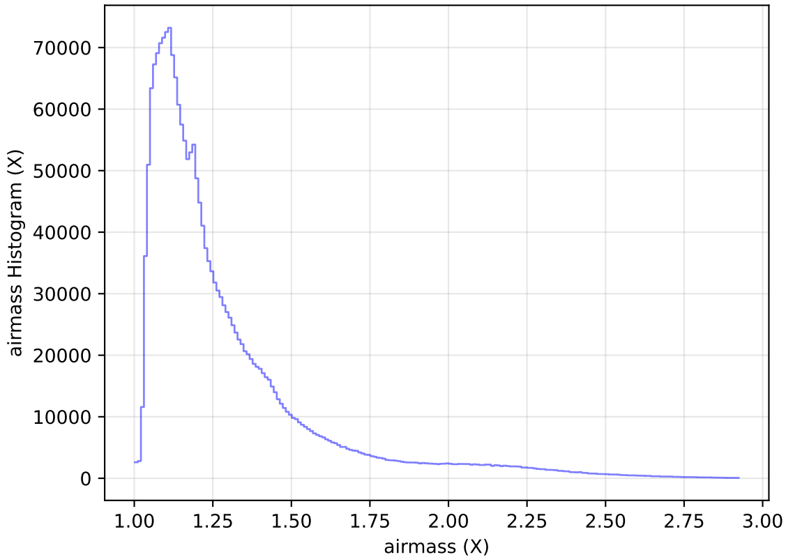
ddf_acor_sf15_lsf40_lsr10_v3.4_10yrs WFD all bands: airmass Histogram
