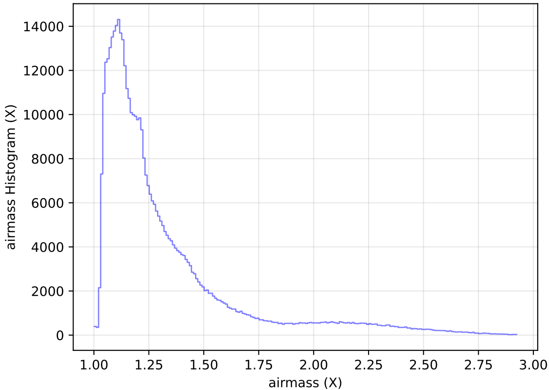
ddf_acor_sf15_lsf40_lsr10_v3.4_10yrs All sky z band: airmass Histogram
