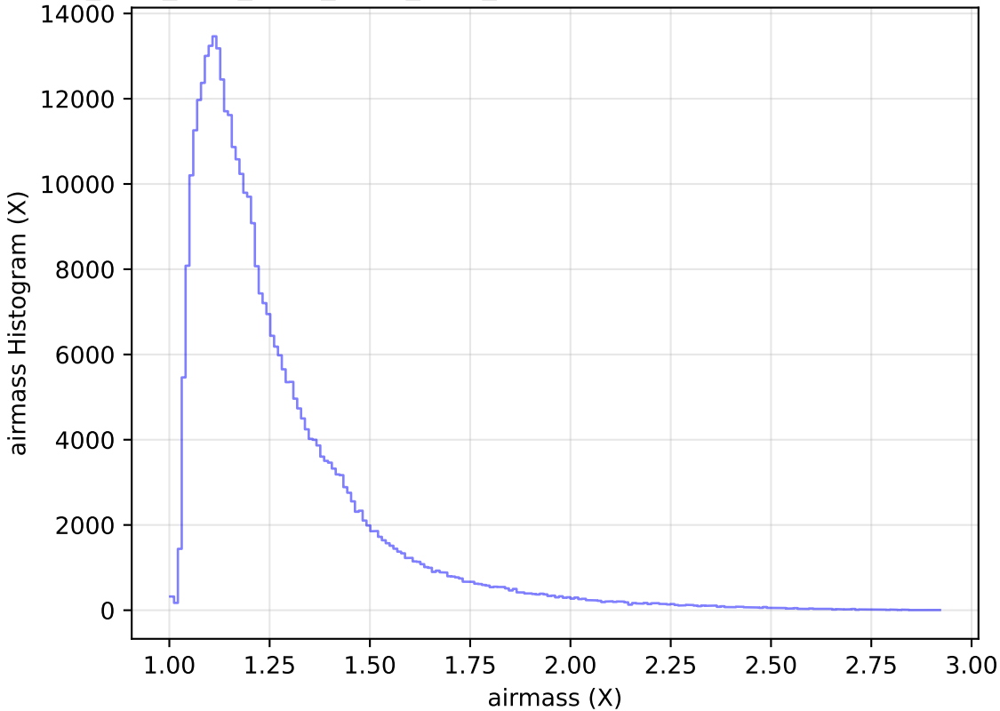
ddf_acor_sf15_lsf40_lsr10_v3.4_10yrs All sky y band: airmass Histogram
