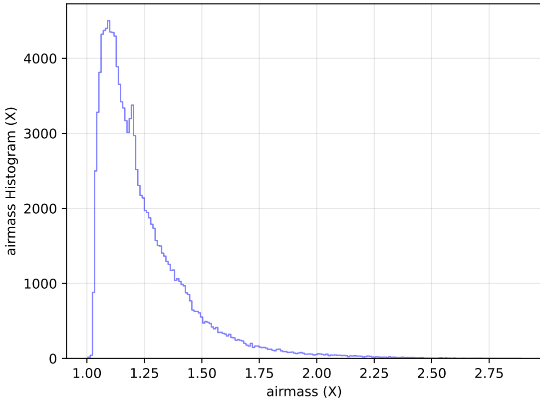
ddf_acor_sf15_lsf40_lsr10_v3.4_10yrs All sky u band: airmass Histogram
