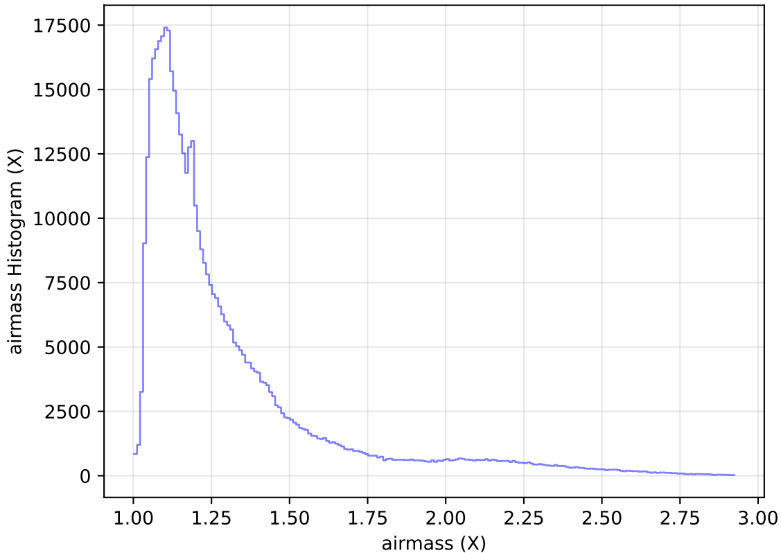
ddf_acor_sf15_lsf40_lsr10_v3.4_10yrs All sky i band: airmass Histogram
