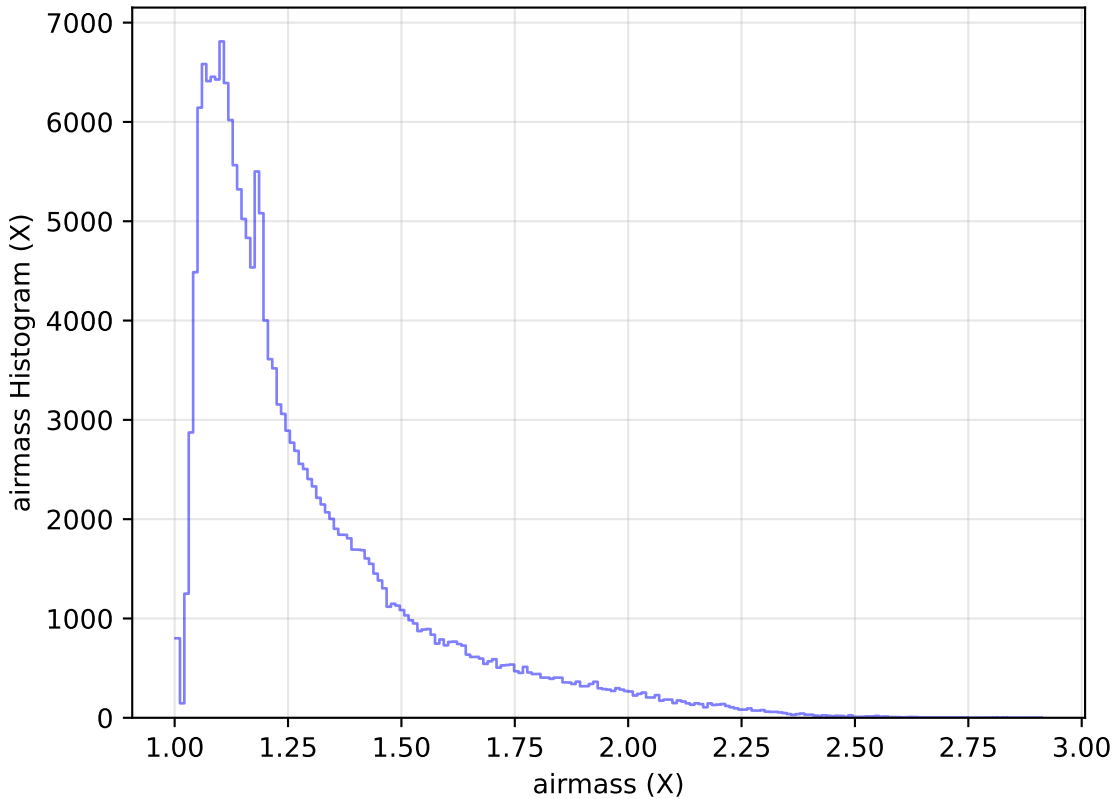
ddf_acor_sf15_lsf40_lsr10_v3.4_10yrs All sky g band: airmass Histogram
