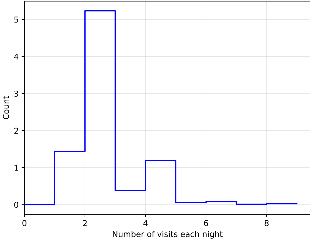
ddf_acor_sf15_lsf40_lsr10_v3.4_10yrs WFD: NVisitsPerNight 1e6
