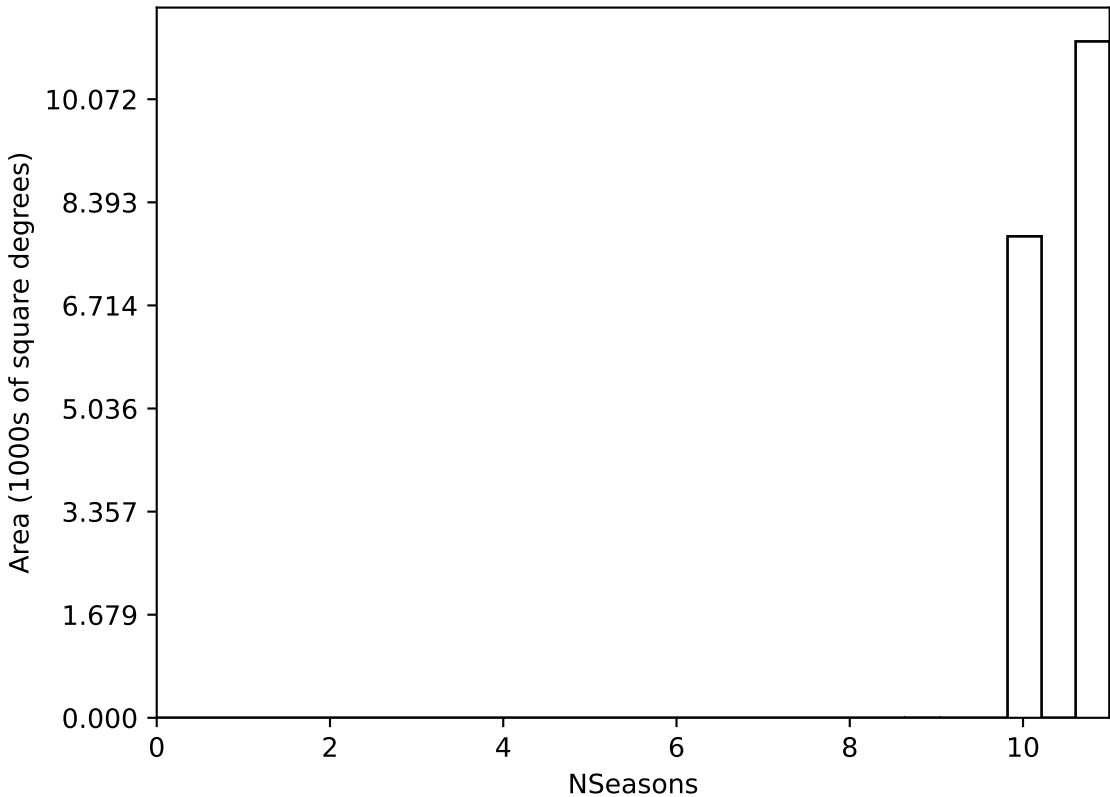
ddf_acor_sf15_lsf40_lsr10_v3.4_10yrs WFD all bands: NSeasons
