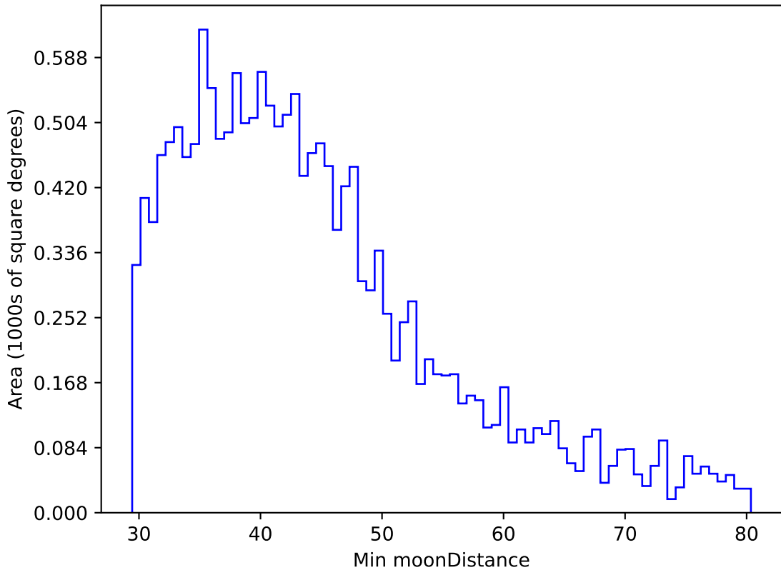
ddf_acor_sf15_lsf40_lsr10_v3.4_10yrs WFD g band: Min moonDistance
