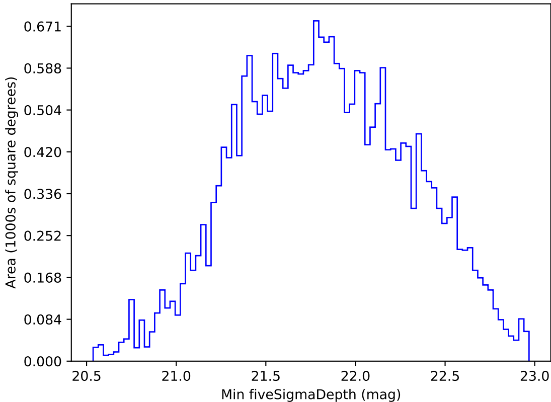
ddf_acor_sf15_lsf40_lsr10_v3.4_10yrs All sky i band: Min fiveSigmaDepth
