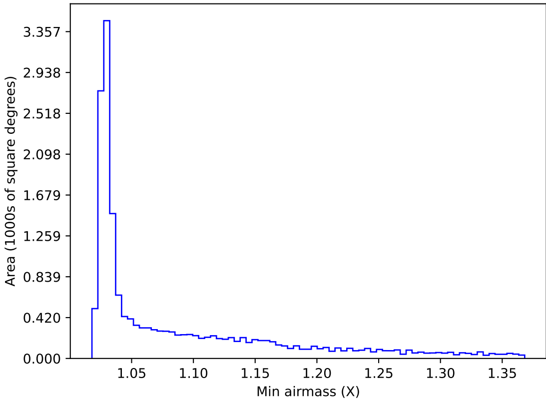
ddf_acor_sf15_lsf40_lsr10_v3.4_10yrs WFD z band: Min airmass
