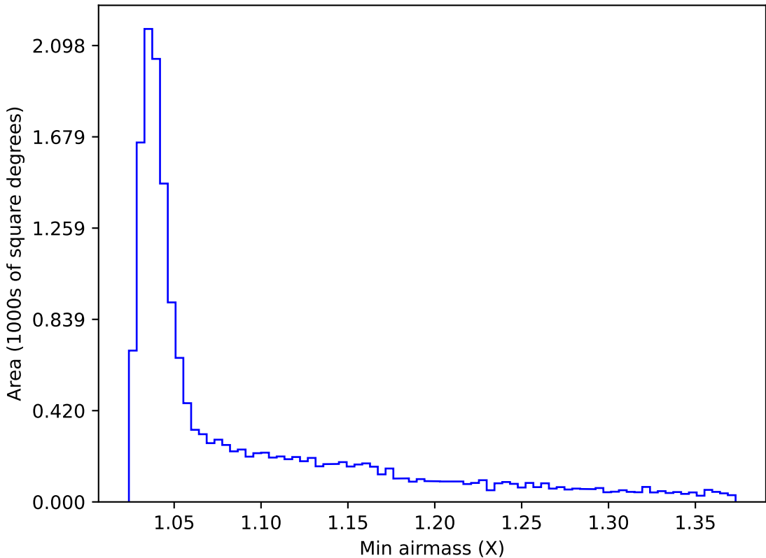
ddf_acor_sf15_lsf40_lsr10_v3.4_10yrs WFD u band: Min airmass
