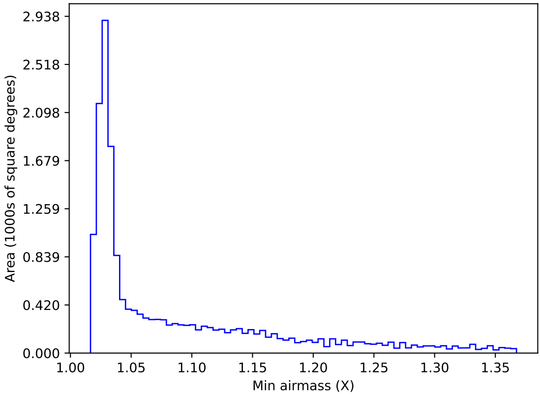
ddf_acor_sf15_lsf40_lsr10_v3.4_10yrs WFD r band: Min airmass
