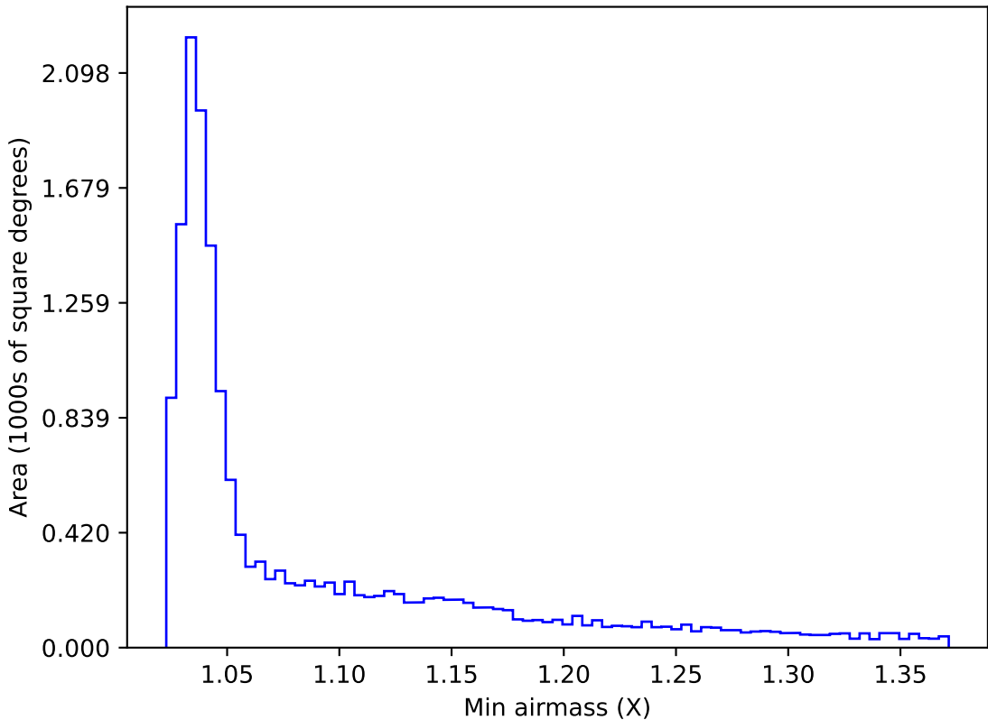
ddf_acor_sf15_lsf40_lsr10_v3.4_10yrs WFD g band: Min airmass
