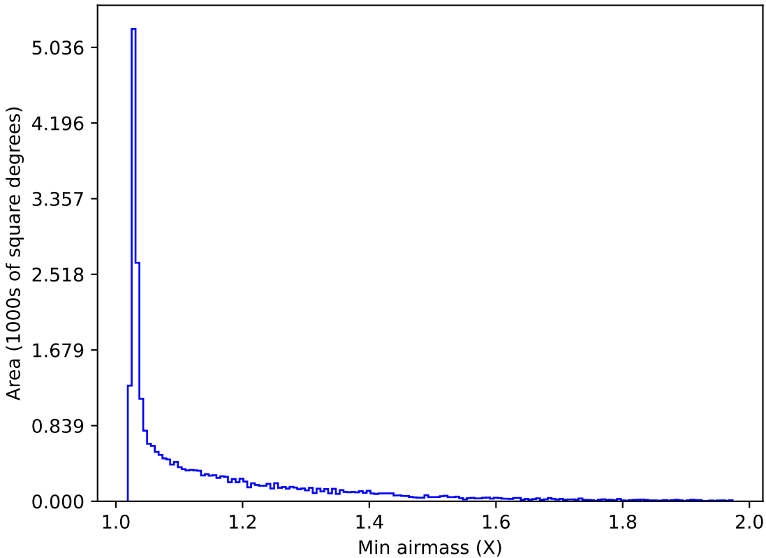
ddf_acor_sf15_lsf40_lsr10_v3.4_10yrs All sky z band: Min airmass
