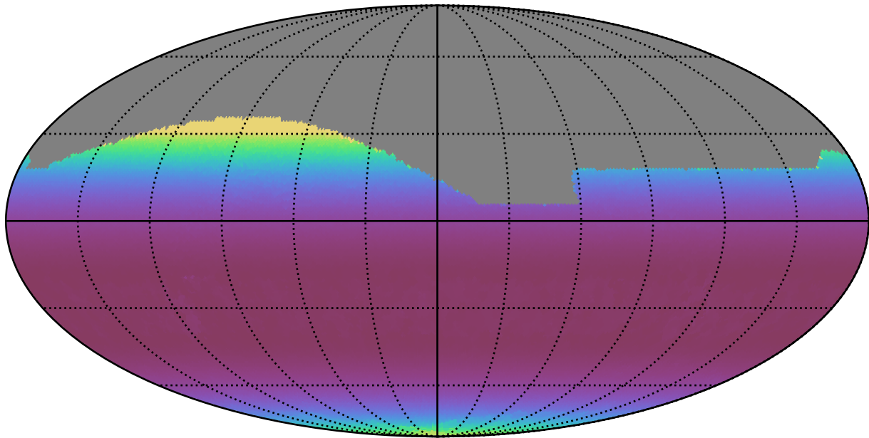
ddf_acor_sf15_lsf40_lsr10_v3.4_10yrs All sky r band: Min airmass
