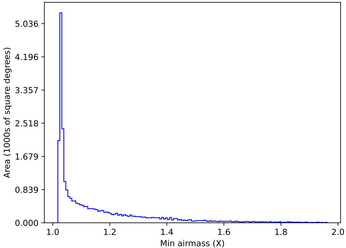
ddf_acor_sf15_lsf40_lsr10_v3.4_10yrs All sky i band: Min airmass
