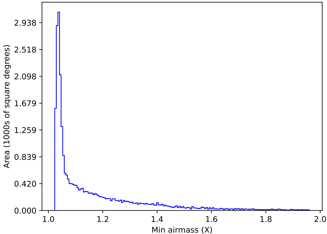
ddf_acor_sf15_lsf40_lsr10_v3.4_10yrs All sky g band: Min airmass
