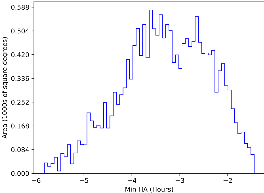
ddf_acor_sf15_lsf40_lsr10_v3.4_10yrs WFD u band: Min HA
