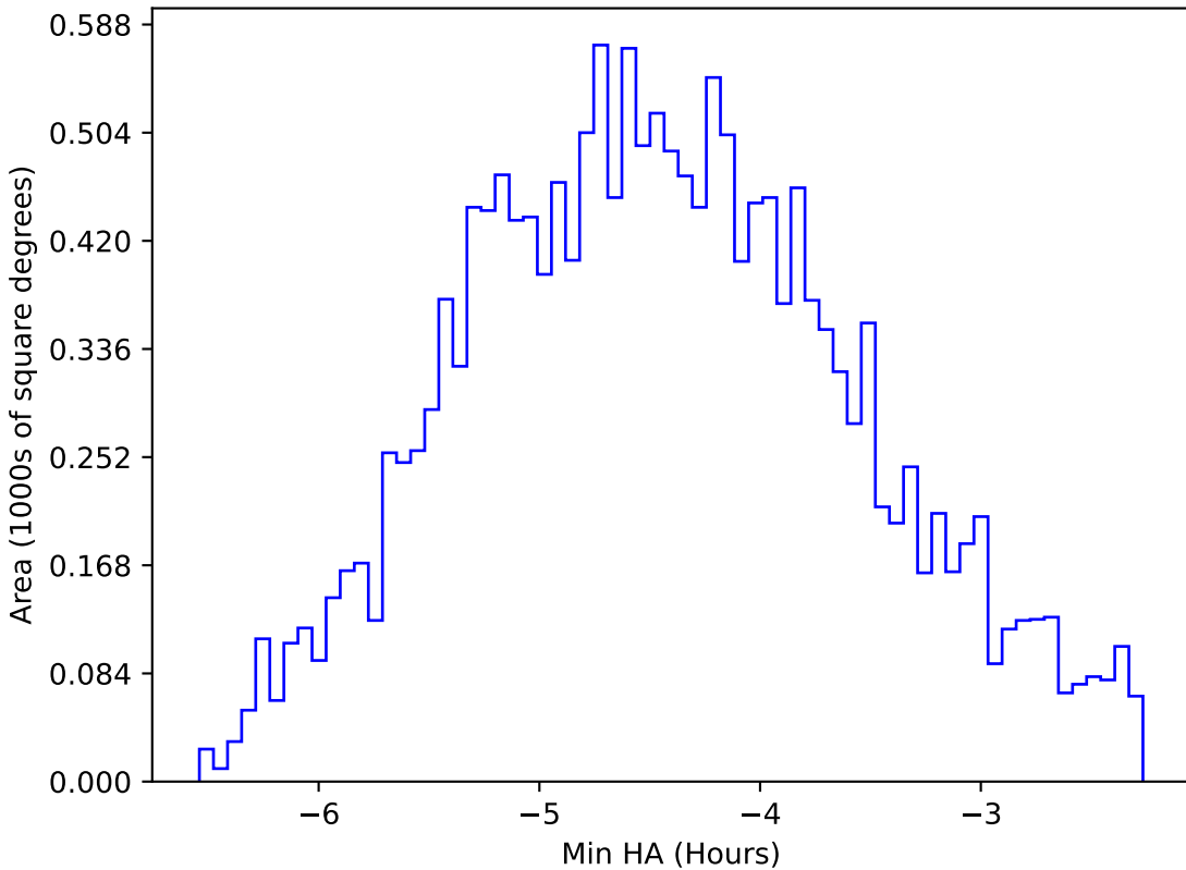
ddf_acor_sf15_lsf40_lsr10_v3.4_10yrs WFD r band: Min HA
