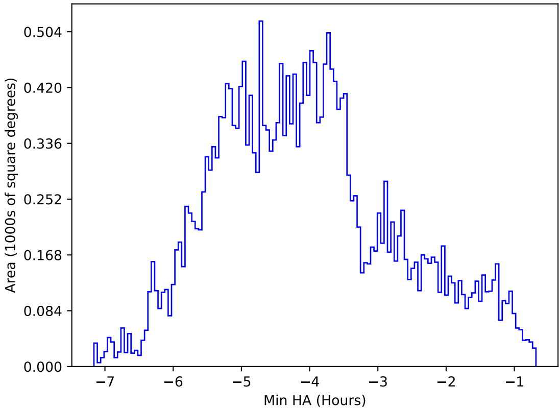
ddf_acor_sf15_lsf40_lsr10_v3.4_10yrs All sky z band: Min HA
