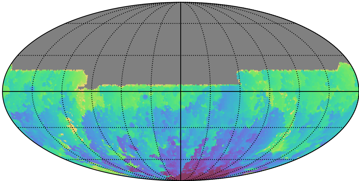
ddf_acor_sf15_lsf40_lsr10_v3.4_10yrs All sky u band: Min HA
