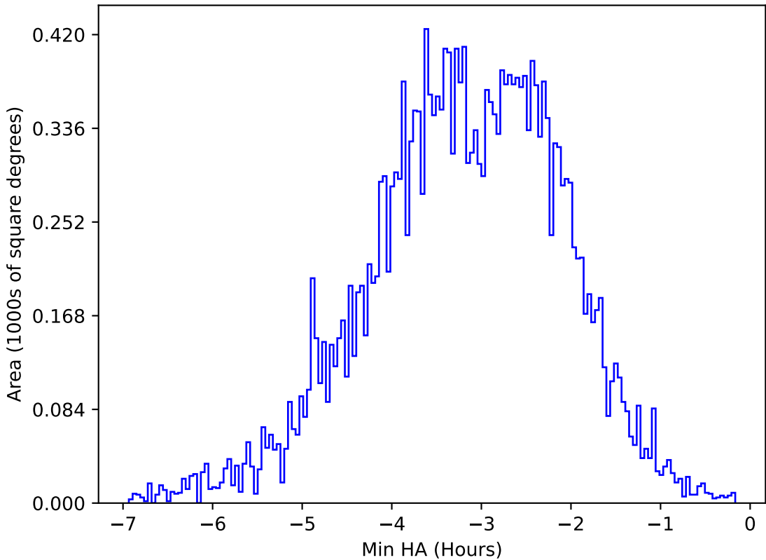
ddf_acor_sf15_lsf40_lsr10_v3.4_10yrs All sky u band: Min HA
