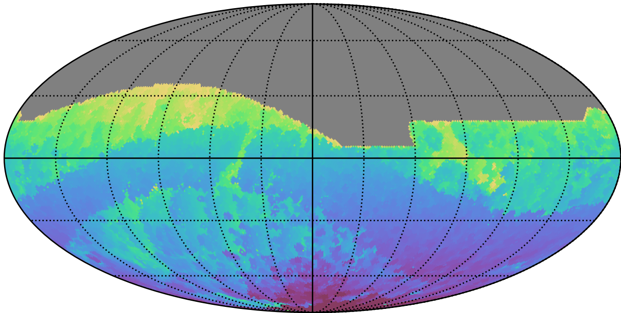
ddf_acor_sf15_lsf40_lsr10_v3.4_10yrs All sky r band: Min HA
