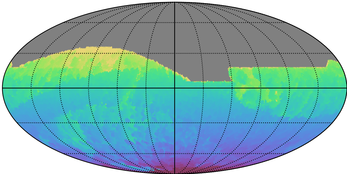
ddf_acor_sf15_lsf40_lsr10_v3.4_10yrs All sky all bands: Min HA
