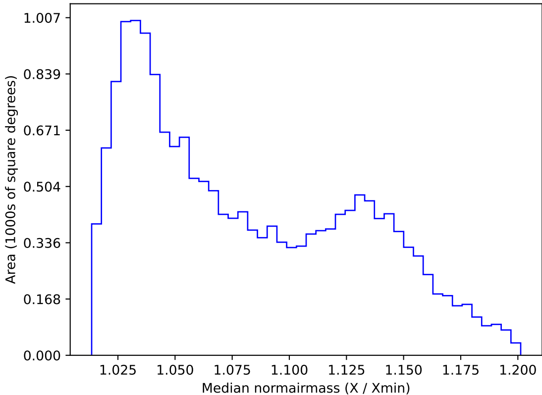
ddf_acor_sf15_lsf40_lsr10_v3.4_10yrs WFD g band: Median normairmass
