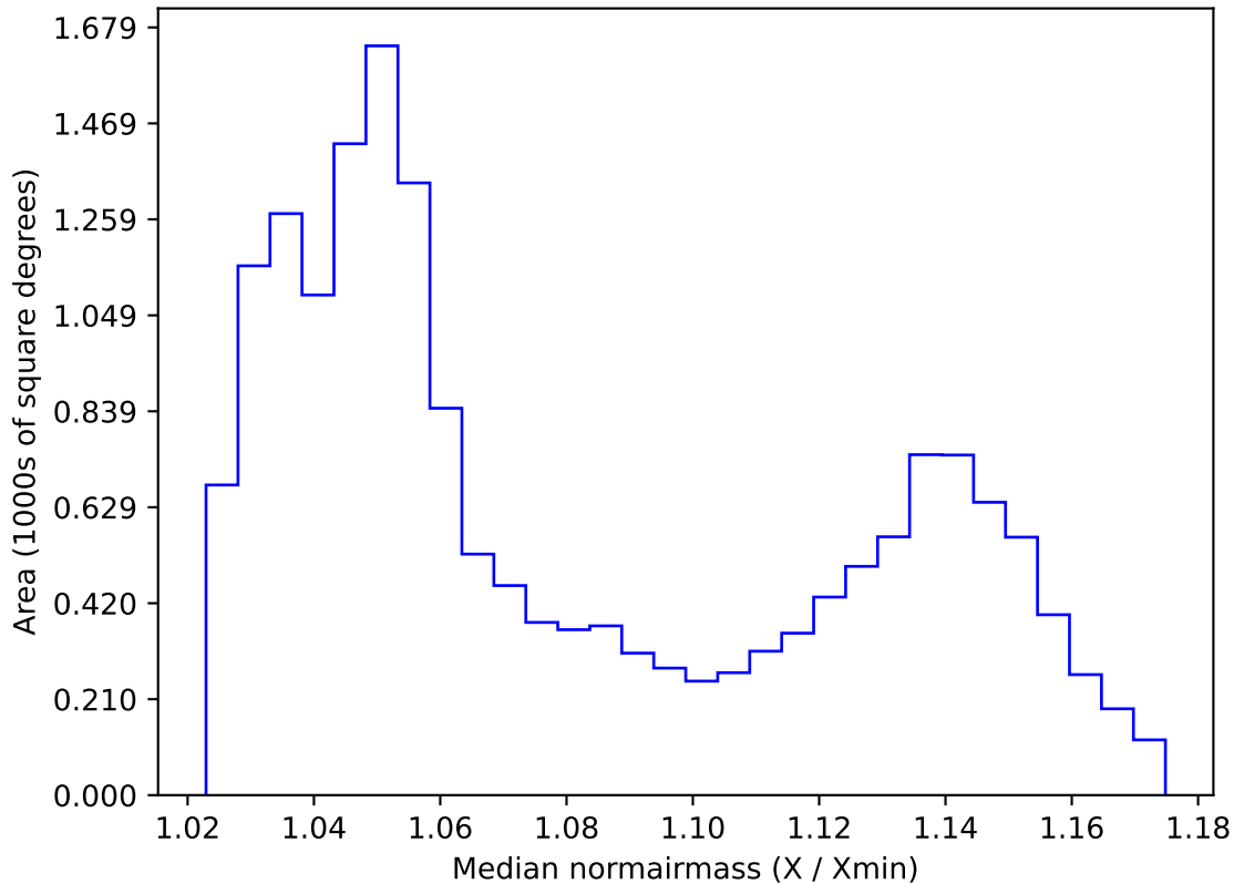
ddf_acor_sf15_lsf40_lsr10_v3.4_10yrs WFD all bands: Median normairmass
