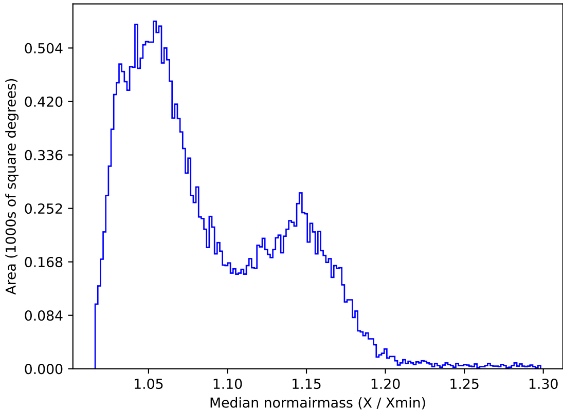
ddf_acor_sf15_lsf40_lsr10_v3.4_10yrs All sky z band: Median normairmass
