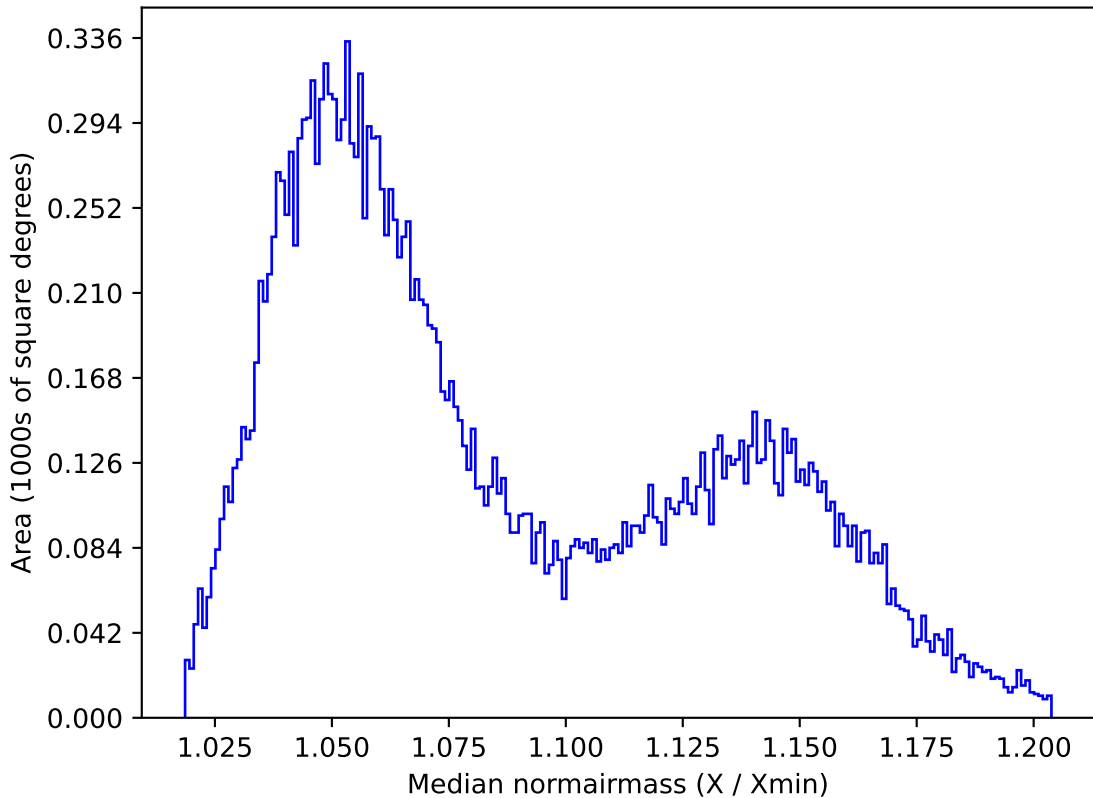
ddf_acor_sf15_ls40_lsr10_v3.4_10yrs All sky y band: Median normairmass
