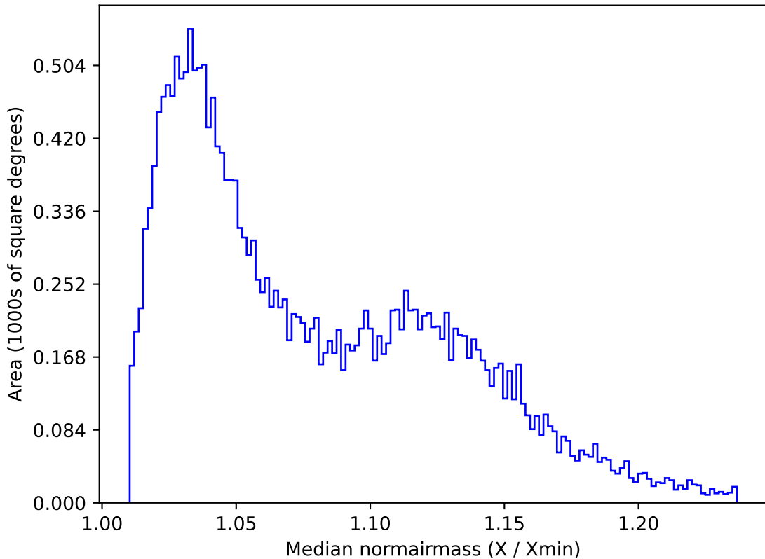
ddf_acor_sf15_ls40_lsr10_v3.4_10yrs All sky u band: Median normairmass
