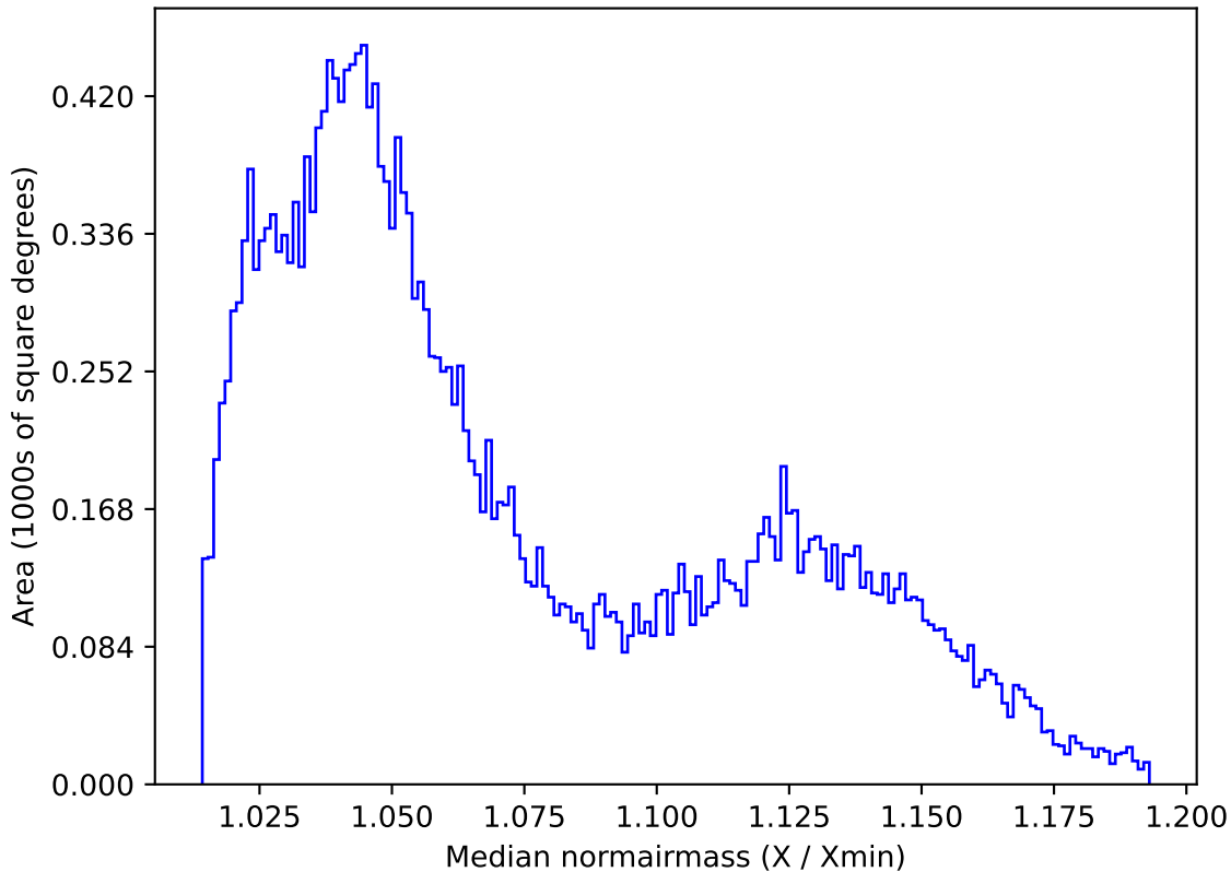
ddf_acor_sf15_lsf40_lsr10_v3.4_10yrs All sky r band: Median normairmass
