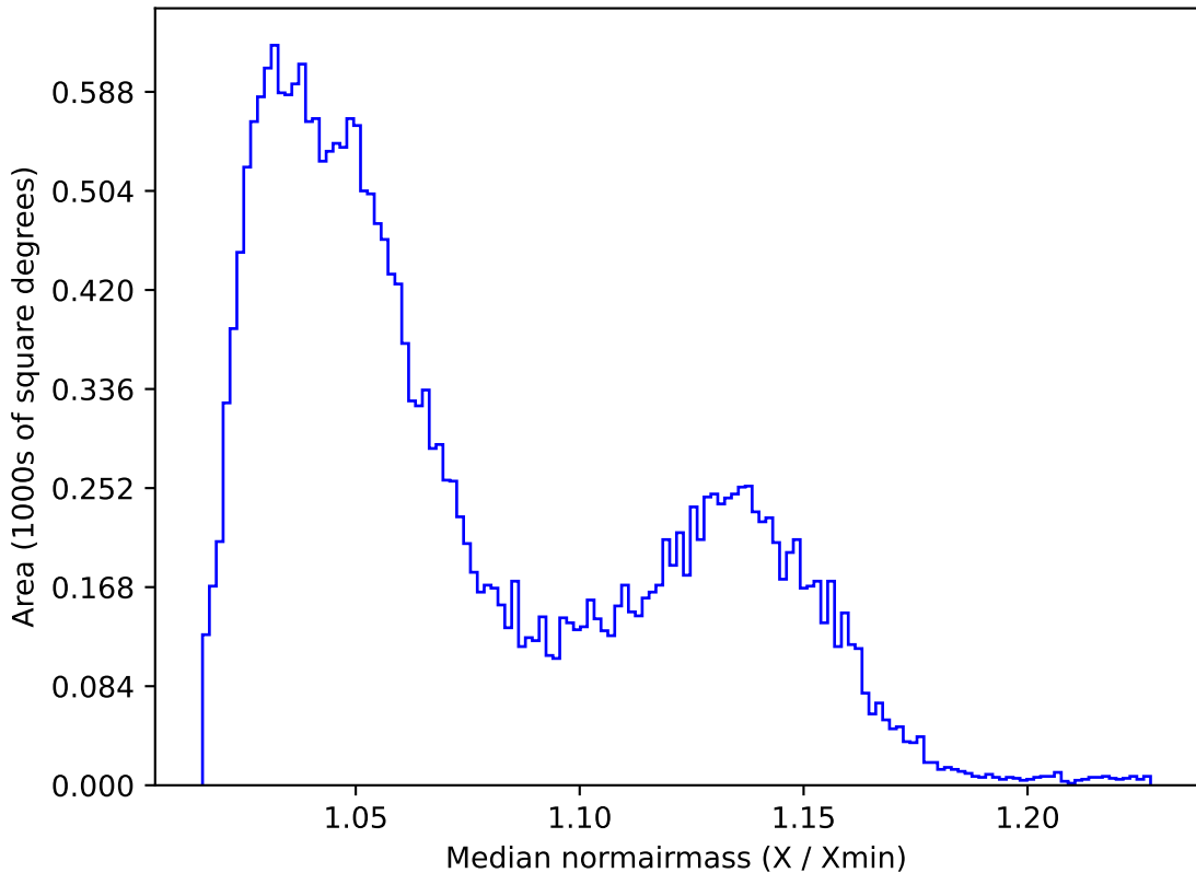
ddf_acor_sf15_lsf40_lsr10_v3.4_10yrs All sky i band: Median normairmass
