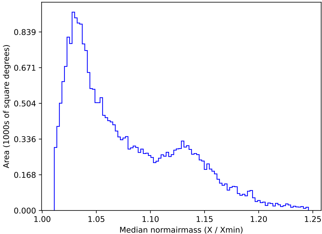
ddf_acor_sf15_ls40_lsr10_v3.4_10yrs All sky g band: Median normairmass
