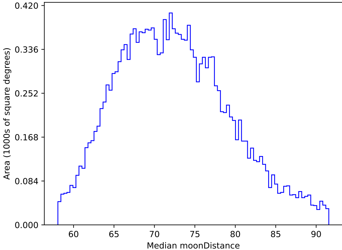
ddf_acor_sf15_lsf40_lsr10_v3.4_10yrs WFD z band: Median moonDistance
