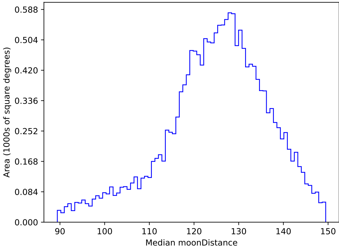
ddf_acor_sf15_lsf40_lsr10_v3.4_10yrs WFD u band: Median moonDistance
